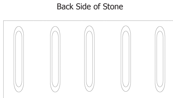
Apply 3/8" to 1/2" Vertical strips of TABS Structural Silicone
